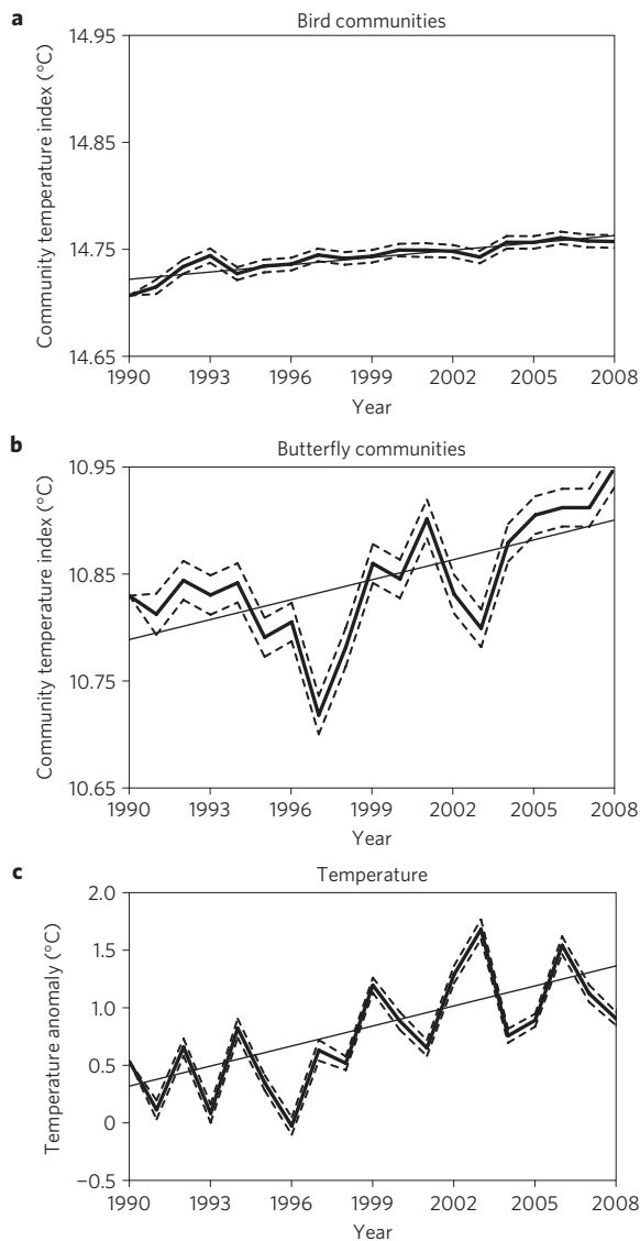
Figure 1 | Temporal trend of CTI and temperature in Europe from 1990 to 2008 ( \pm standard error of the mean in dashed lines). a, b, CTI for the bird (a) and butterfly (b) communities monitored in Europe from 1990 to 2008. c, March–September temperature for the same period. Temperature anomalies are calculated as the departure from the average of the base period 1961–1990.
