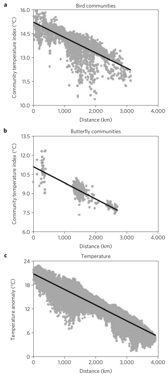
Figure 2 | Spatial trend of CTI and temperature in Europe. a, b, Change in CTI for the bird (a) and butterfly (b) communities from south to north. c, Change in March–September temperature along the same gradient. For birds and butterflies, each point represents the CTI for a given sample monitored in 2005. Temperature is the average of March–September temperature to match the breeding season of birds and butterflies. Distance (x axis) is calculated from the southern border of the studied region.
